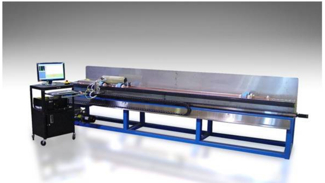
Ultrasonic C-Scan Technology used to verify bond integrity on planar and rotatable bonds
